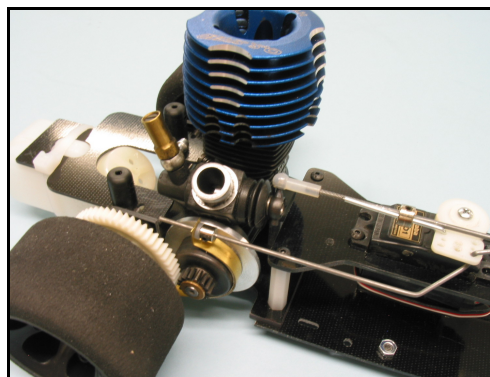
PICTURE OF TYPICAL ENGINE/CLUTCH INSTALLATION
