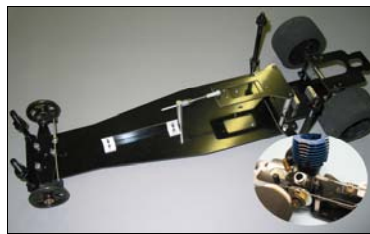
FUNNY CAR CHASSIS AND TYPICAL ENGINE / CLUTCH INSTALLATION SHOWN
